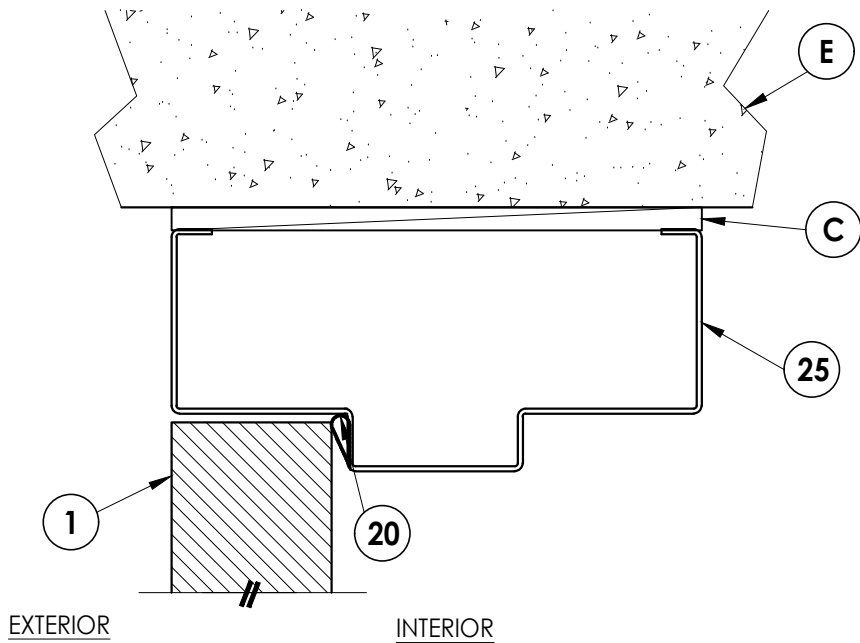
1/7 VERTICAL CROSS SECTION
