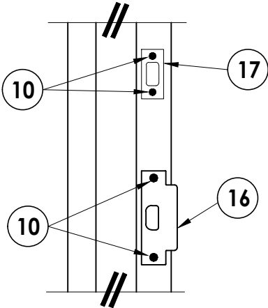
DETAIL 2
