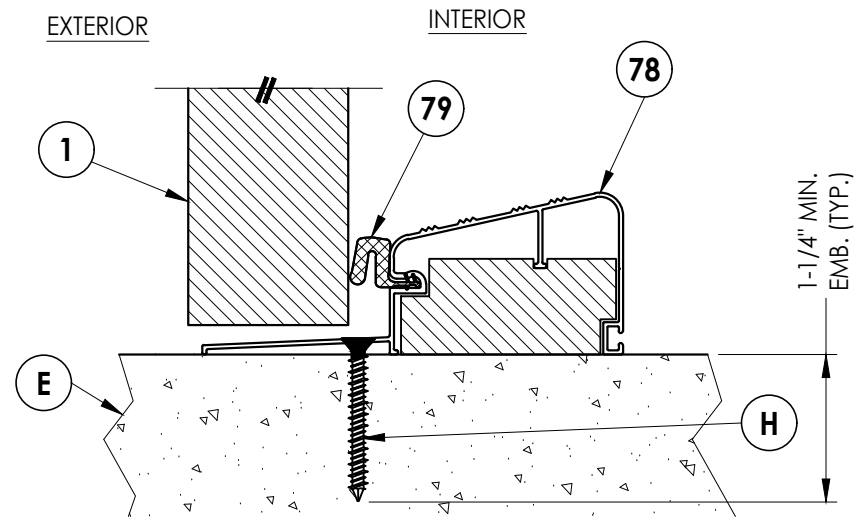
5/7 VERTICAL CROSS SECTION Outswing configuration see general notes, sheet 1 for "HVHZ" water infiltration requirements
