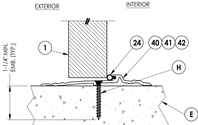
3/7 VERTICAL CROSS SECTION Outswing configuration see general notes, sheet 1 for "HVHZ" water infiltration requirements
