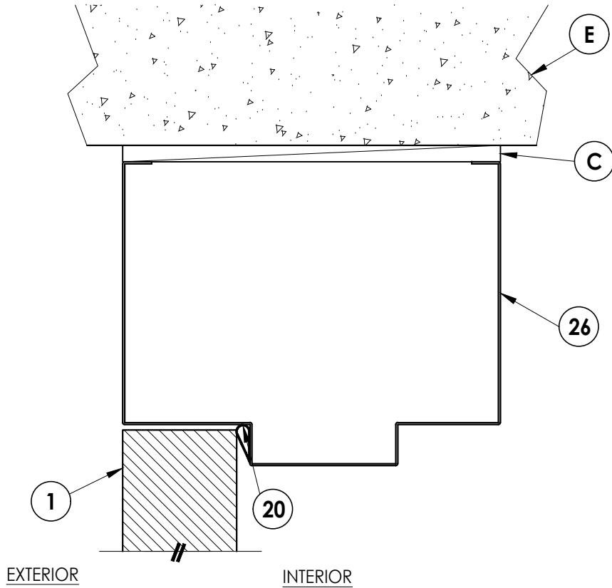
2/7 VERTICAL CROSS SECTION
